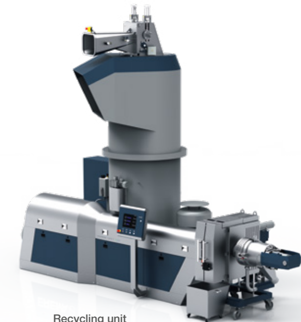
Recycling unit
